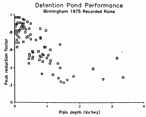
Figure 45. DETPOND modeled peak reduction factors by standard pond for various rain depths and intensities.
