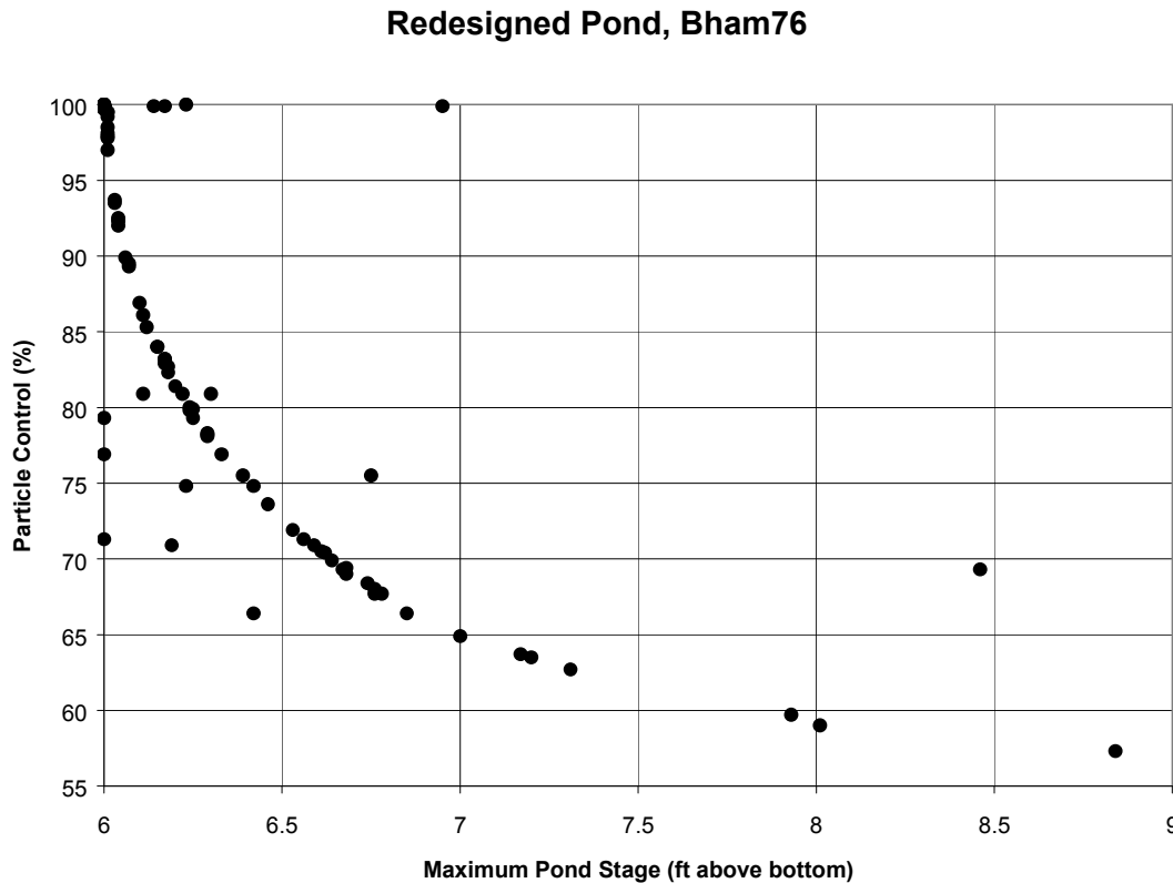
Figure 66. Pond Stage v. Particle Residue Control
