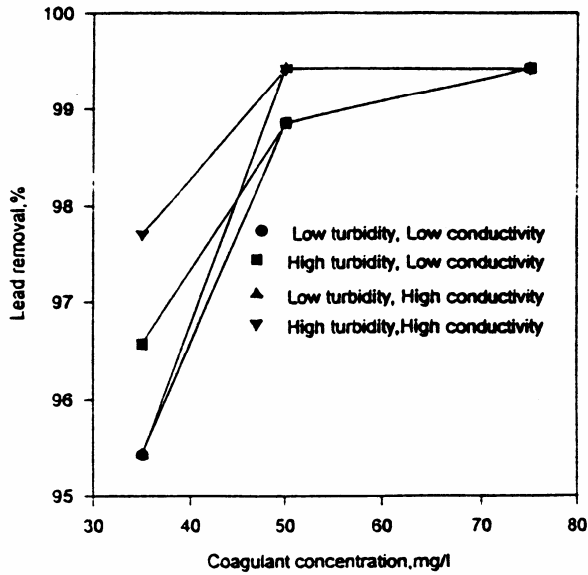
Figure 1. Lead removal using ferric chloride.
