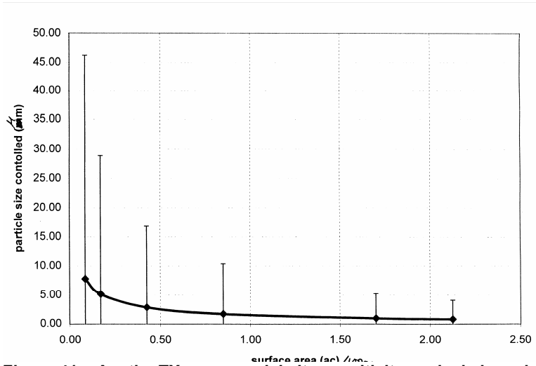
Figure 41a. Austin, TX, commercial site sensitivity analysis based on surface area of pond.
