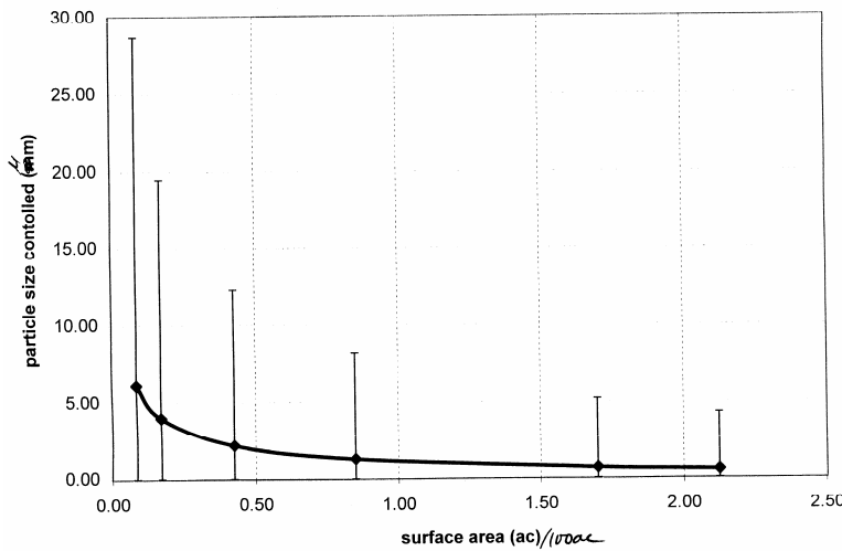
Figure 41b. Minneapolis, MN, commercial area sensitivity analysis based on surface area of pond.
