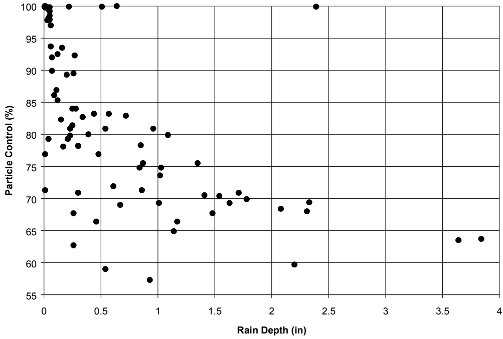
Figure 67. Rain Depth v. Particle Residue Control
