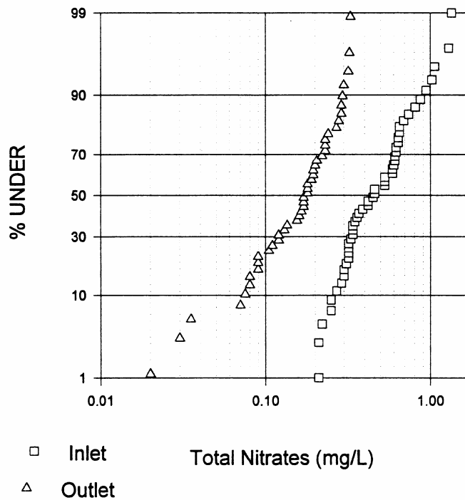
Figure 54. Probability plots of influent and effluent pollutant concentrations.
