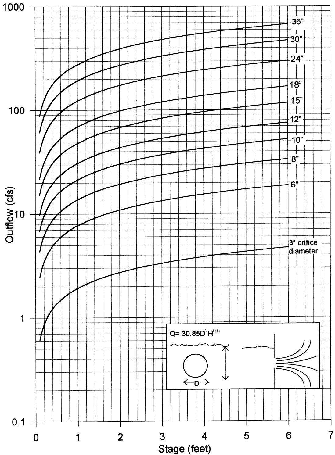
Figure 34. Approximate rating curves for orifice discharges.
