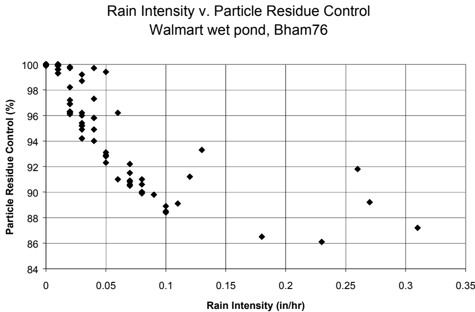
Figure 61. Rain Intensity v. Particle Residue Control
