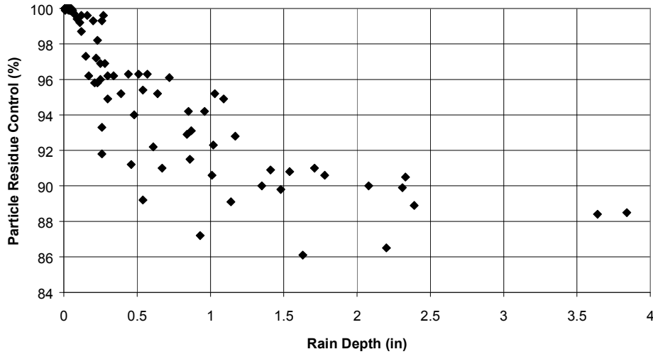
Rain Depth v. Particle Residue Control Walmart wet pond, Bham76
