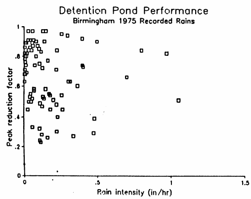
Figure 45. DETPOND modeled peak reduction factors by standard pond for various rain depths and intensities.
